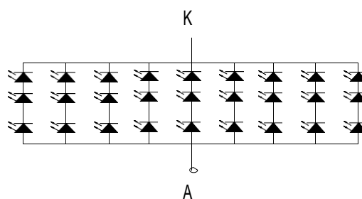
Figure : LED connection of backlight
